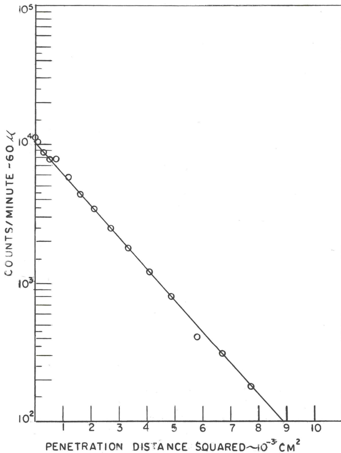
Figure 4. Solute Penetration Curve, Sample No. 59-- Annealed at 24 kb. pressure and 713°K for 3.6 \times 10^3 sec
